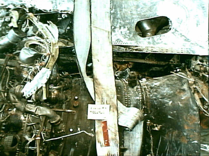
Powerplants 8 - Photo 32. Engine No. 3, left side and pylon.
