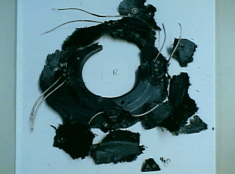
Powerplants 8 - Photo 31. Right propeller bulkhead and electrical leads
