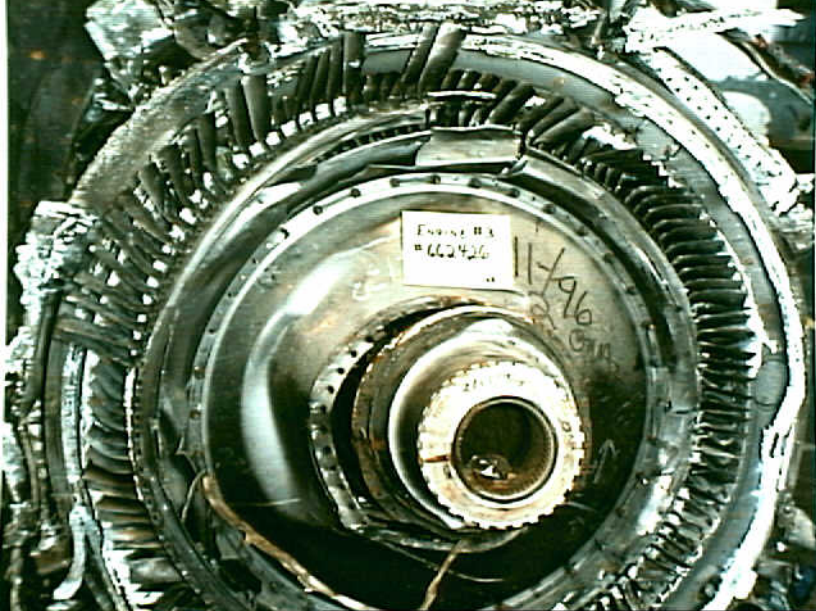
Powerplants 8 - Photo 31. Engine No. 3, showing fan hub and front of LPC, with second and third stage compressor blades bent over away from the direction of rotation.
