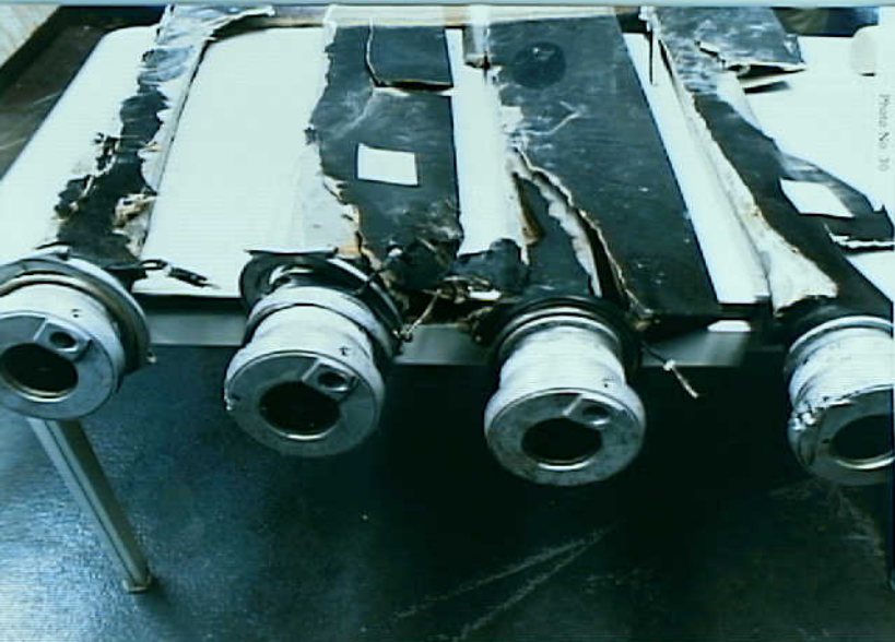
Powerplants 8 - Photo 30. Right propeller blades showing damage to leading edge and missing deicing
