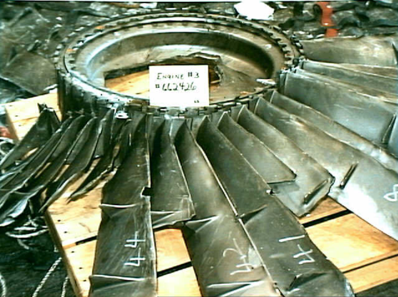
Powerplants 8 - Photo 30. Engine No. 3, fan disk and blades.
