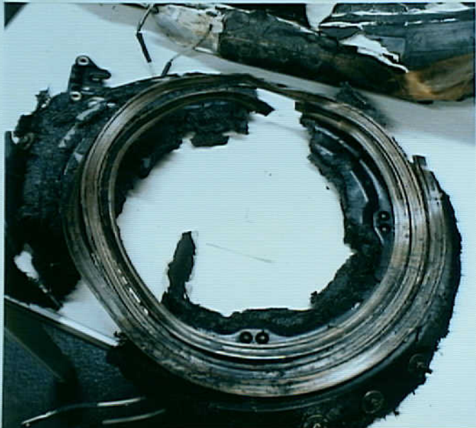
Powerplants 8 - Photo 29. Left propeller slip rings
