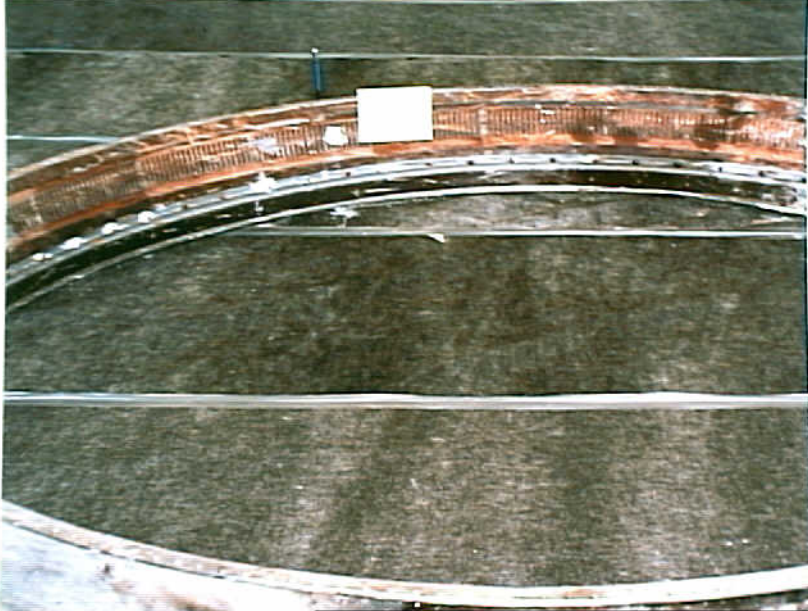
Powerplants 8 - Photo 28. Engine No. 3, upper half of fan rub strip.
