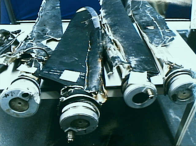
Powerplants 8 - Photo 27. Left propeller blades showing deicing boots
