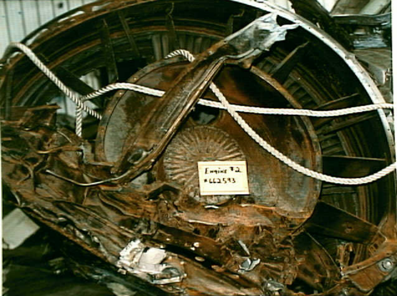
Powerplants 8 - Photo 26. Engine No. 2, turbine exhaust case and No. 4 bearing support with bearing housing cover in place.
