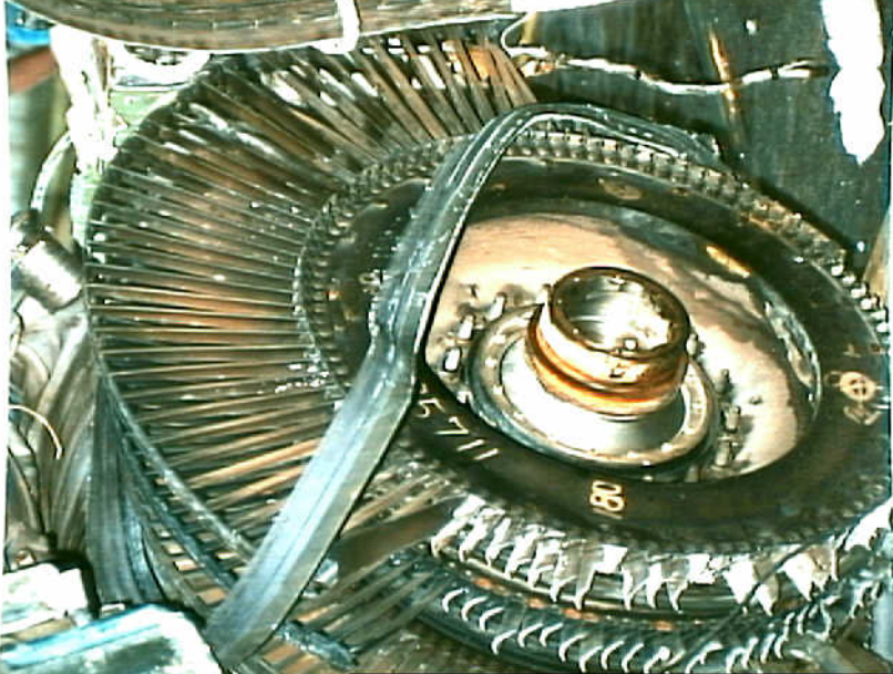
Powerplants 8 - Photo 25. Engine No. 2, rear, showing fourth stage turbine blades, fifth stage turbine hub and blades, and sixth stage turbine disk and blades.
