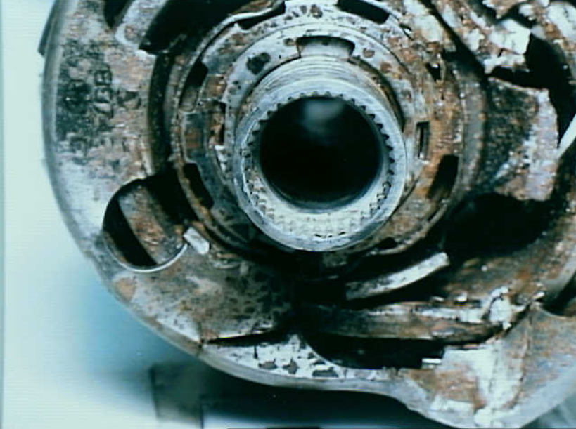
Powerplants 8 - Photo 24. Left propeller servo piston ball screw internal splines
