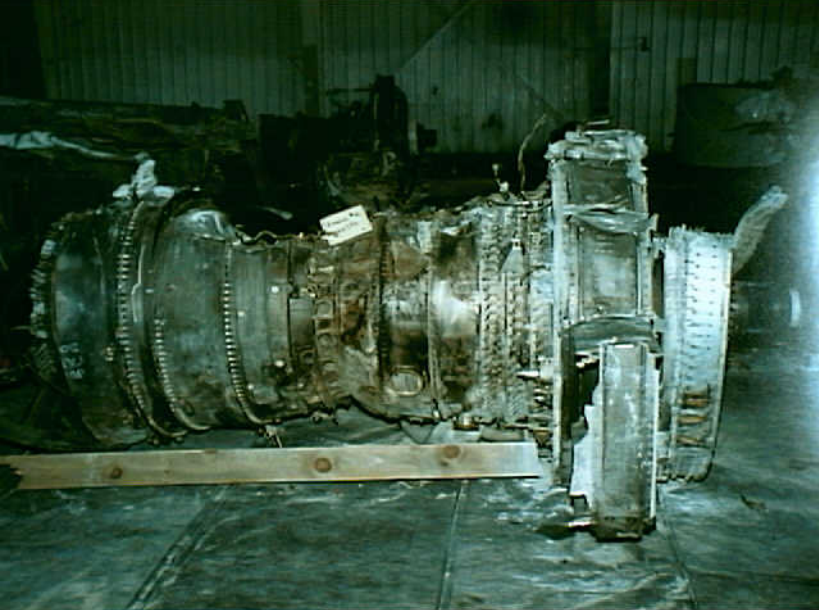
Powerplants 8 - Photo 24. Engine No. 2, bottom
