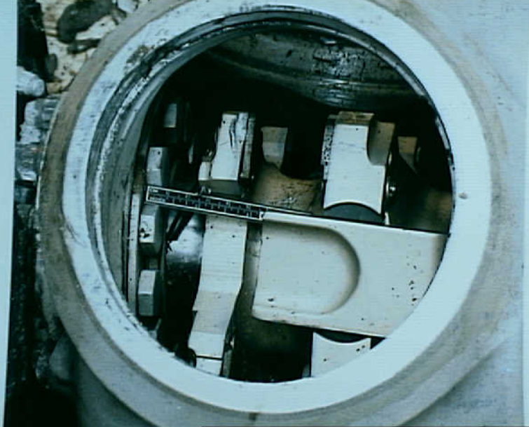
Powerplants 8 - Photo 23. Measurement of yoke to mounting pad flange to determine propeller blade pitch angle
