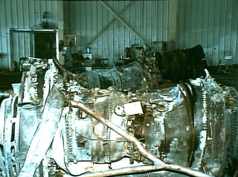
Powerplants 8 - Photo 23. Engine No. 2, top.
