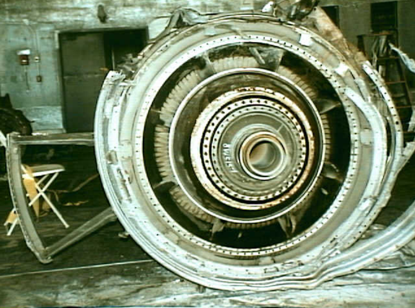
Powerplants 8 - Photo 22. Engine No. 2, front of HPC.
