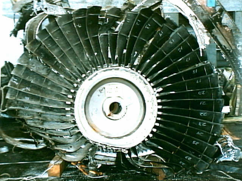
Powerplants 8 - Photo 20. Engine No. 2 fan hub and blades
