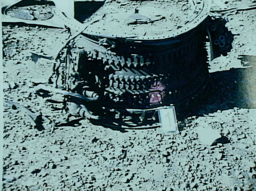
Powerplants 8 - Photo 2. No. 1 engine HPC case half.
