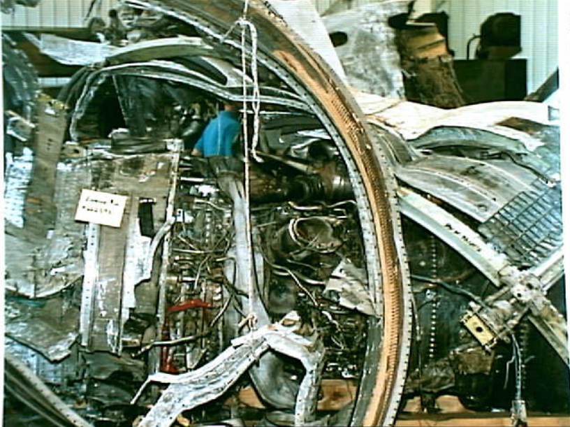
Powerplants 8 - Photo 19. Engine No. 2 fan rub strip and thrust reverser actuator.
