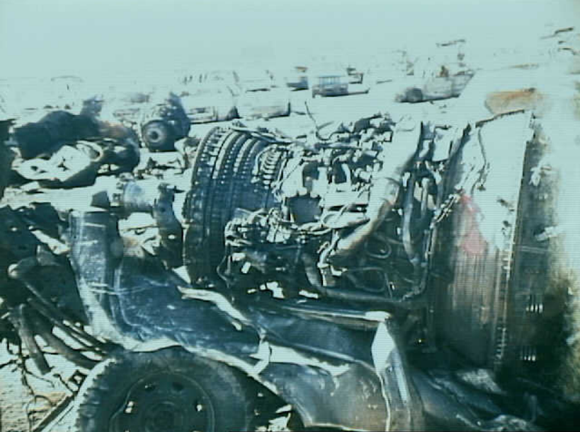
Powerplants 8 - Photo 17. Side view of No. 4 engine from HPC to turbine frame.
