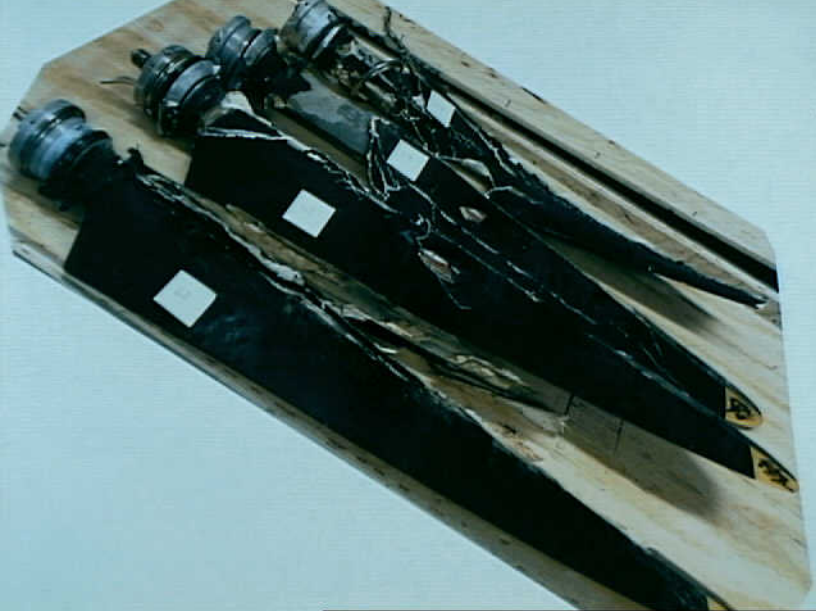
Powerplants 8 - Photo 17. Comparison of the four left propeller blades
