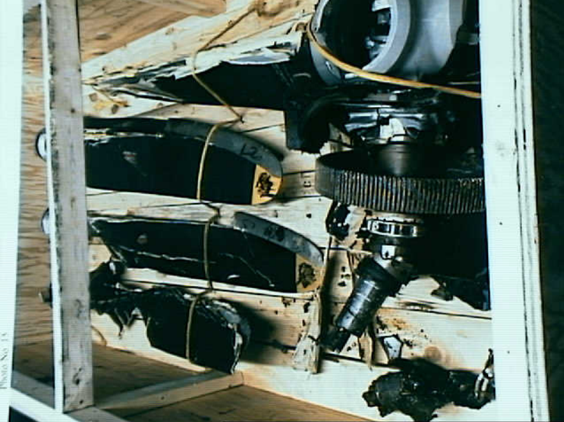
Powerplants 8 - Photo 15. Left propeller assembly as received at Hamilton Standard
