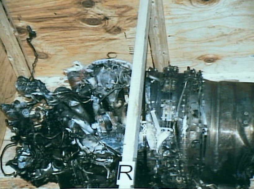
Powerplants 8 - Photo 14. Right engine prepared for shipment to Pratt & Whitney of Canada
