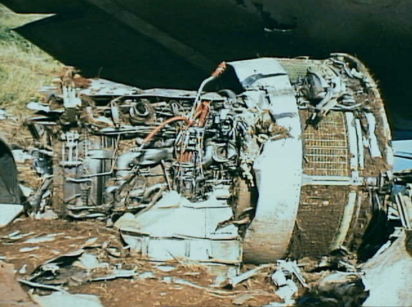
Powerplants 8 - Photo 14. No. 3 engine top and thrust reverser actuators and cascades
