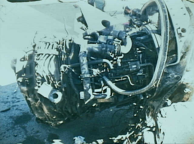
Powerplants 8 - Photo 13. Side view No. 3 engine.
