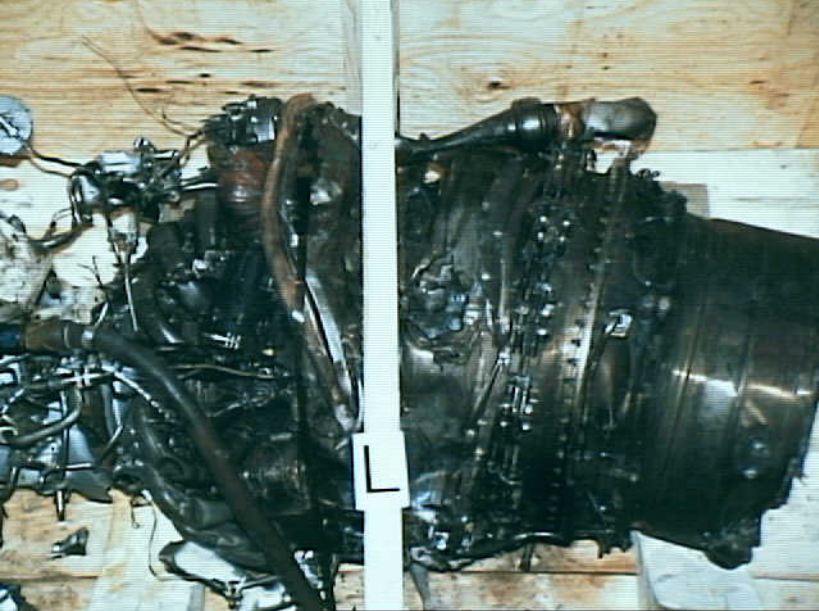
Powerplants 8 - Photo 13. Left engine prepared for shipment to Pratt & Whitney of Canada
