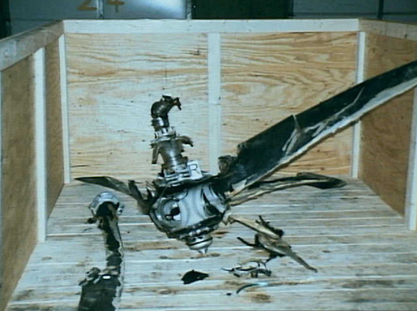
Powerplants 8 - Photo 12. Right propeller assembly prepared for shipment to Hamilton Standard
