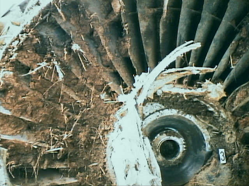
Powerplants 8 - Photo 12. No. 3 engine fan
