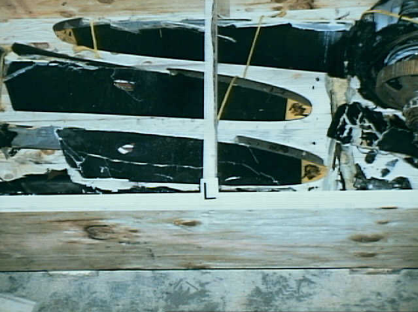
Powerplants 8 - Photo 11. Left propeller assembly prepared for shipment to Hamilton Standard
