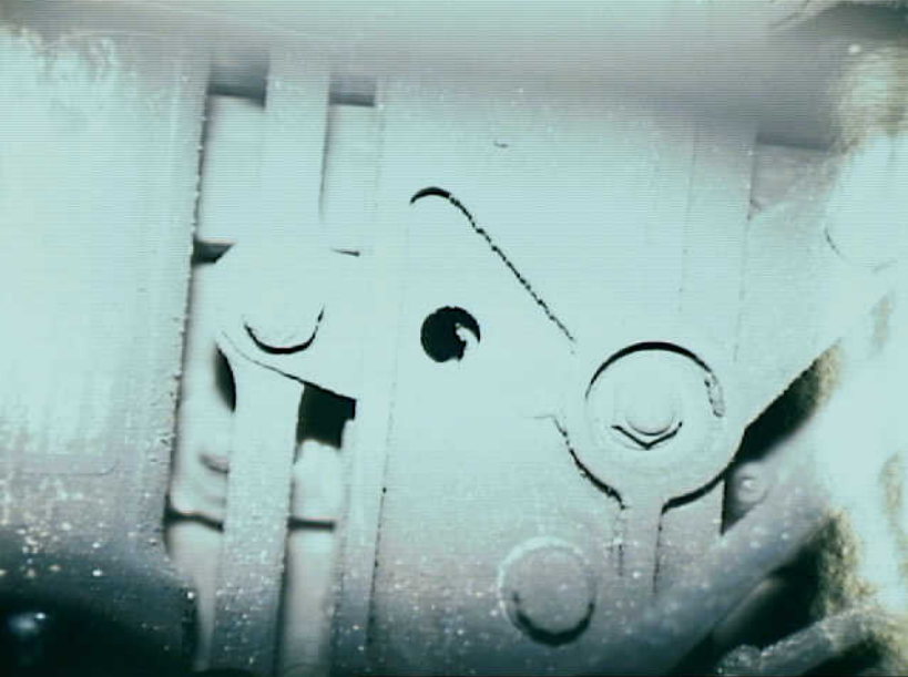
Powerplants 8 - Photo 11. Close up of No. 2 engine VSV showing rig pin hole alignment.
