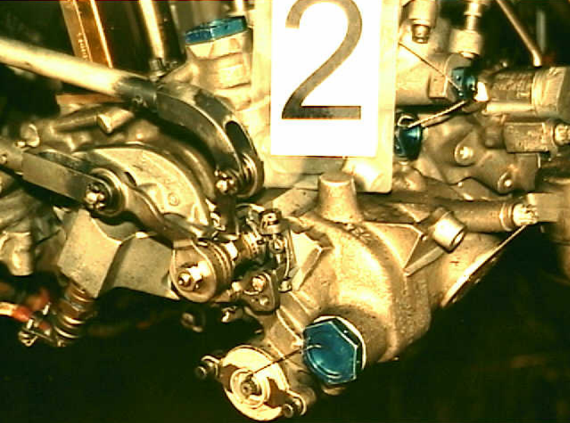
Powerplants 8 - Exhibit No. 8B - Photo 15. No. 2 engine thrust reverser in deployed position.
