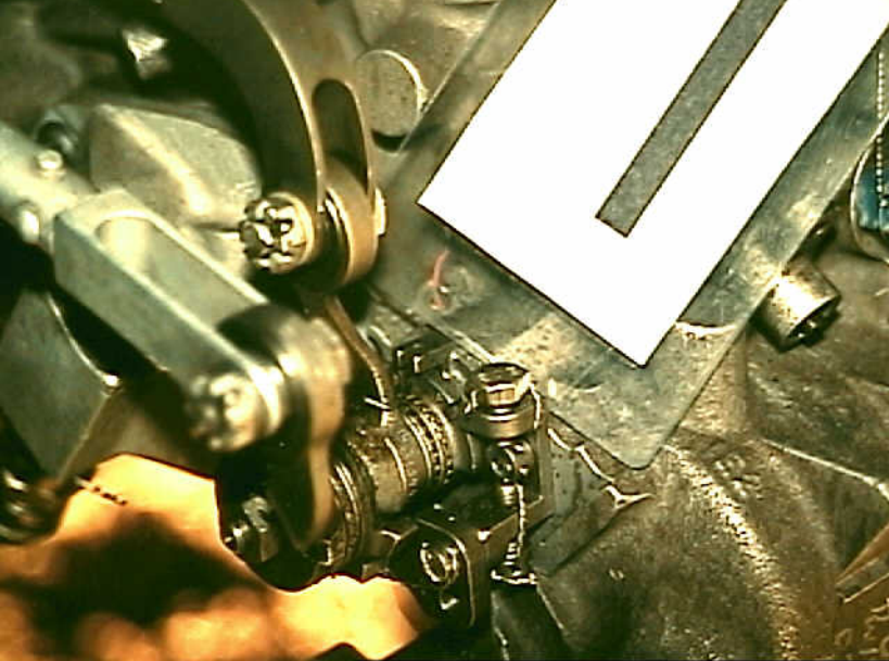
Powerplants 8 - Exhibit No. 8B - Photo 14. No. 1 engine thrust reverser lower door showing mud on interior surface.
