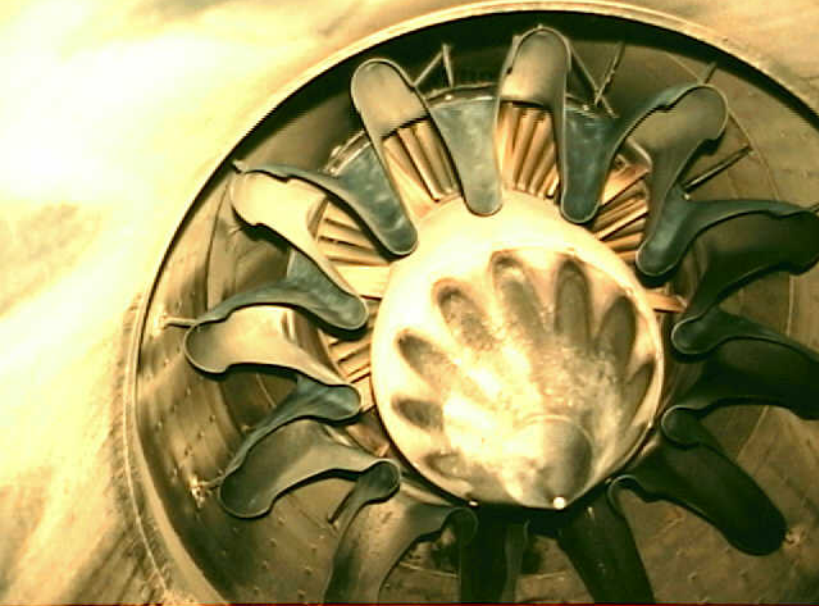
Powerplants 8 - Exhibit No. 8B - Photo 13. No. 1 engine thrust reverser actuator support assembly broken at forward end.
