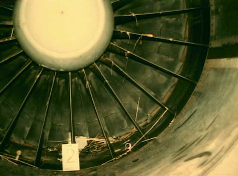
Powerplants 8 - Exhibit No. 8B - Photo 12. Right side of No. 1 engine thrust reverser in deployed position showing damage.
