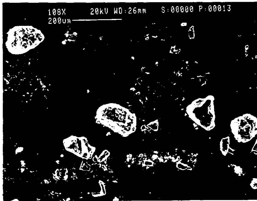
Figure 3. A low magnification SEM view of the majority of particles in the submitted sample. (108X).
