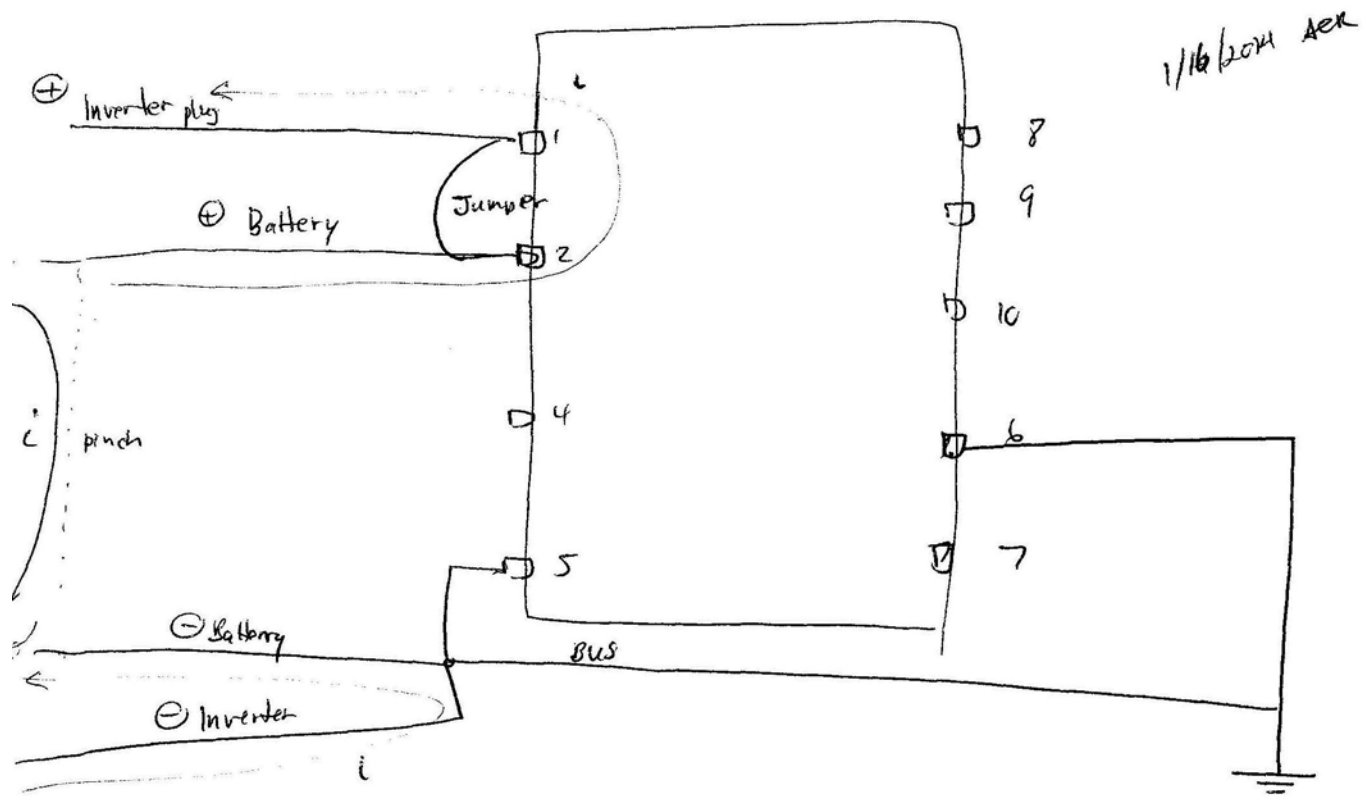
Figure 3 - IMSAR Drawing of Step Up Transformer Wiring
