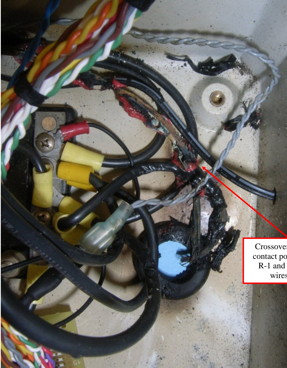
Figure 11 - Grommeted Hole and Damaged Wires
