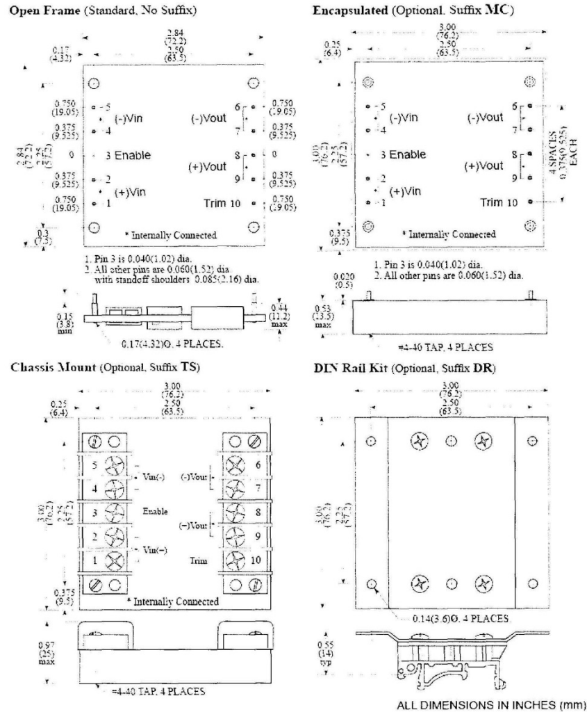
Figure 4 - Manufacturer's Drawing of Step Up Transformer
