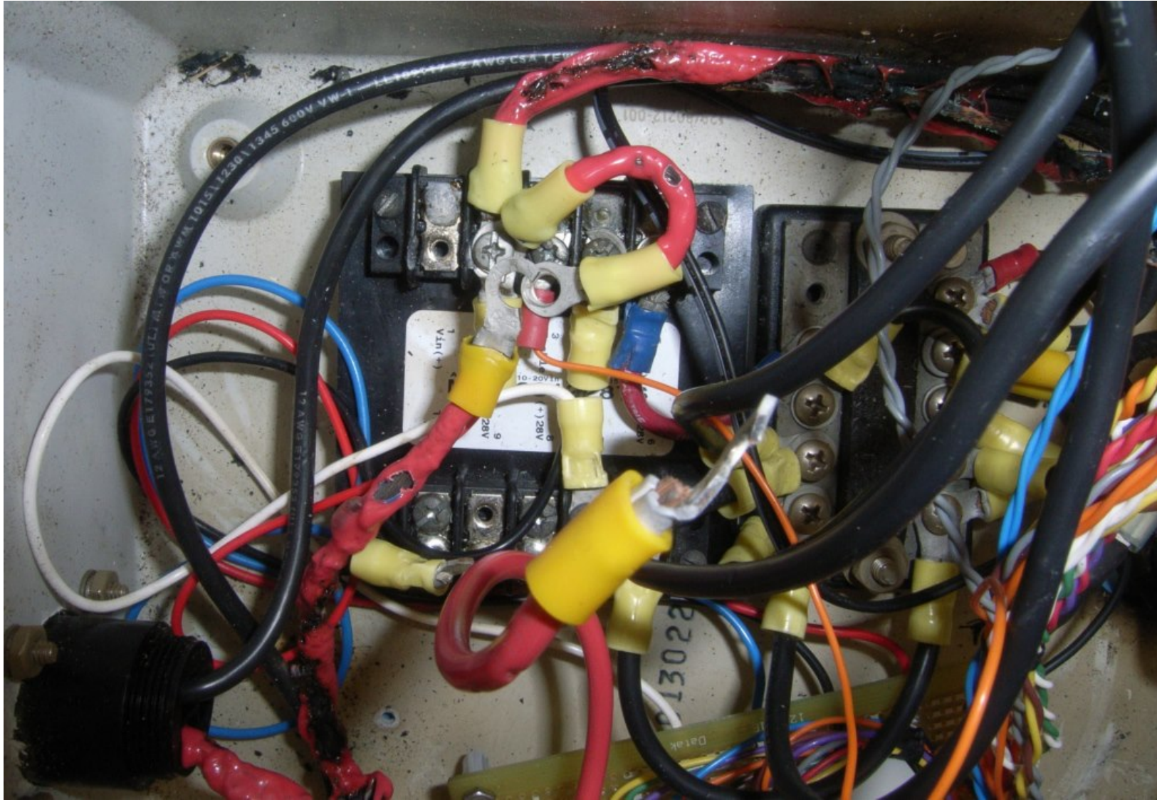
Figure 8 - Step Up Transformer and Bus Block
