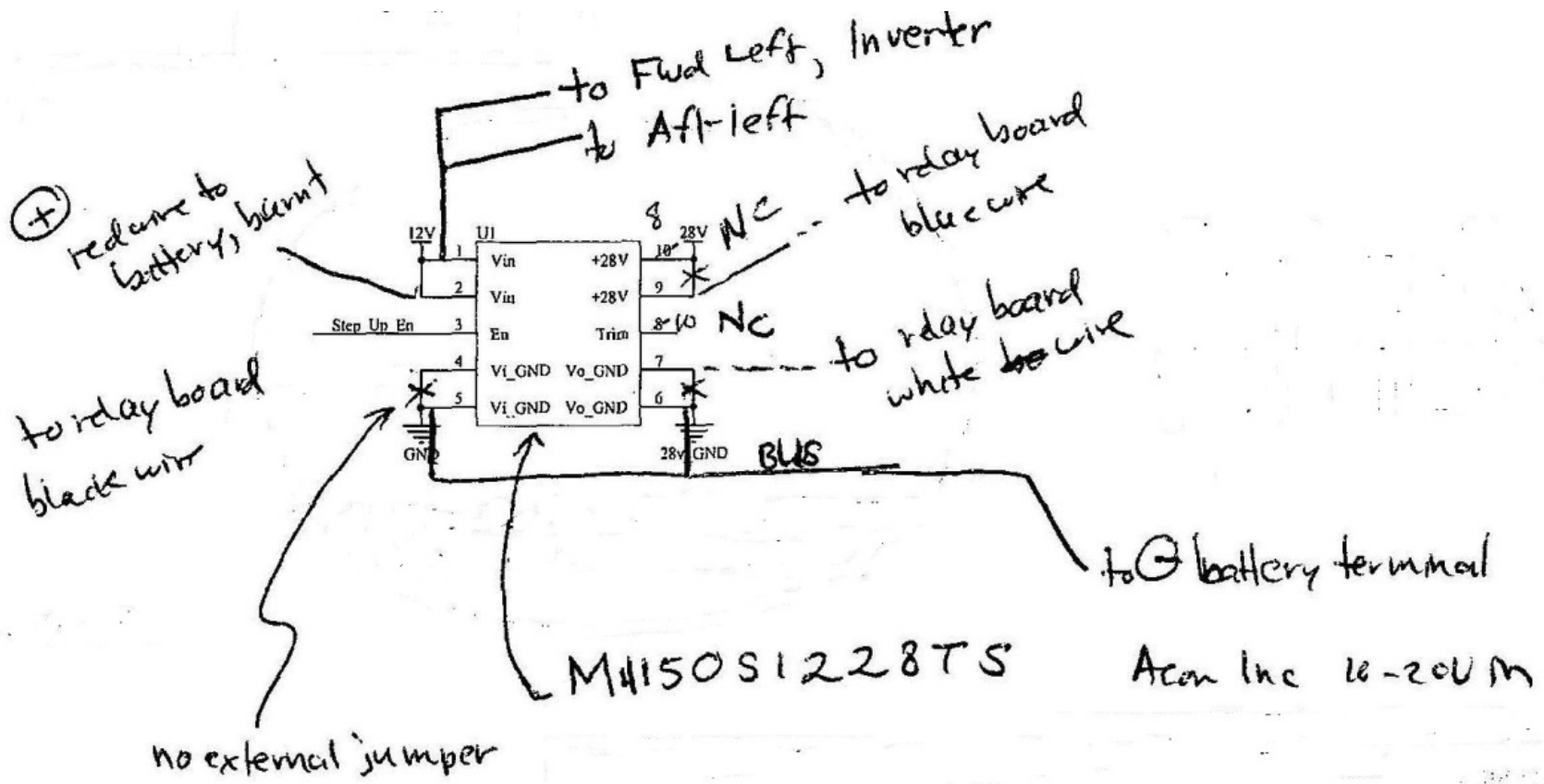
Figure 2 - IMSAR Diagram of Step Up Transformer Wiring
