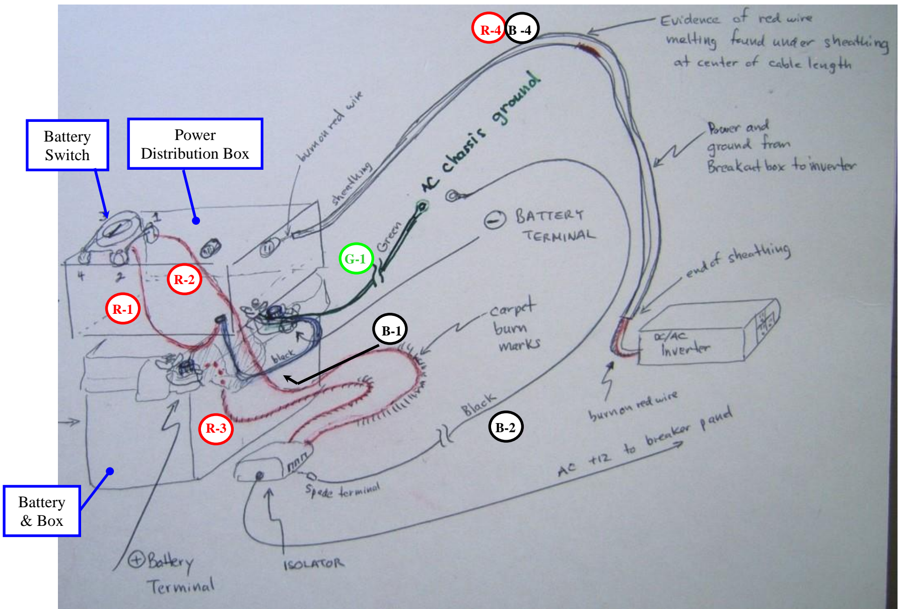
Figure 1 - Supplemental Power System Arrangement and Damage
