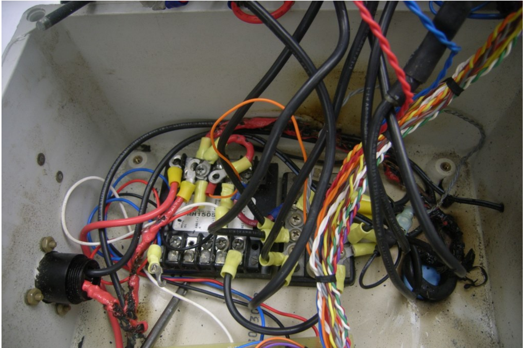
Figure 6 - Step Up Transformer, Bus Block, and Grommeted Hole
