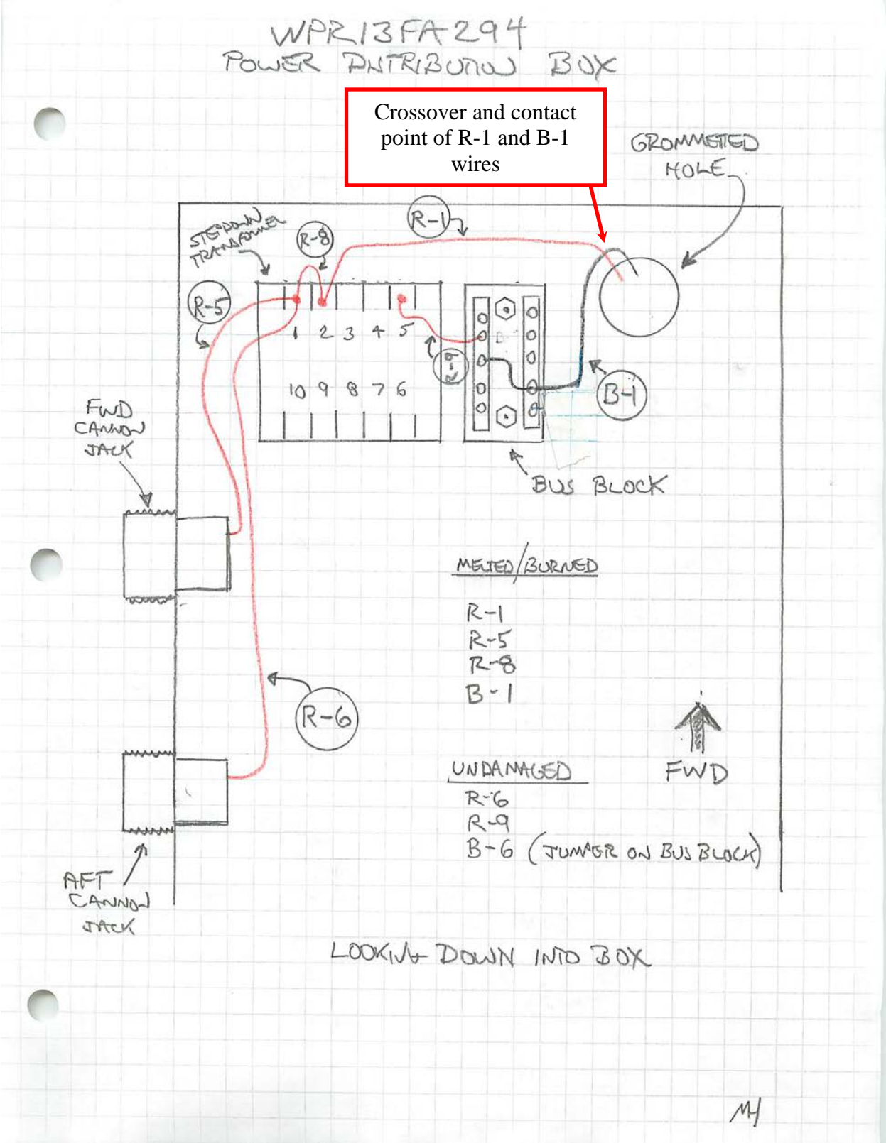
Figure 12 - Diagram of Distribution Box Wiring Damage
