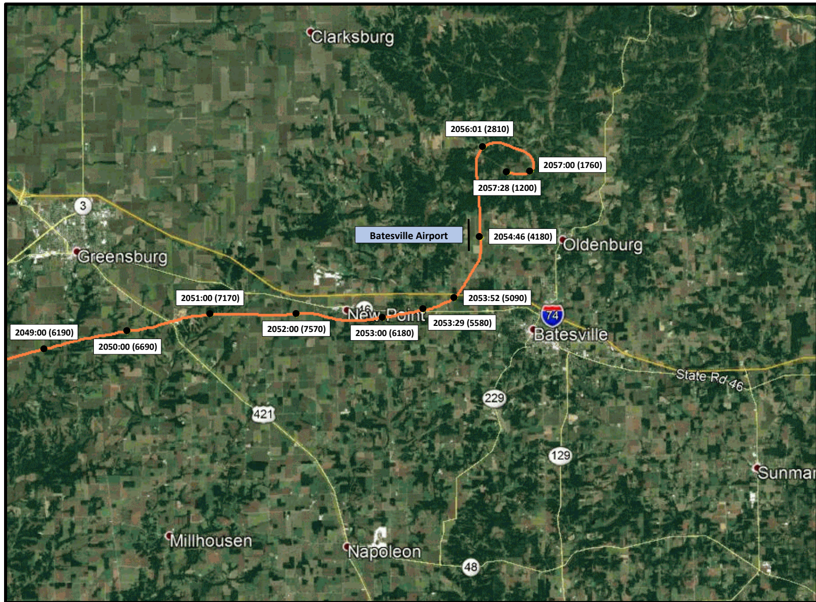
Figure 2 – Final Segment of Accident Flight
