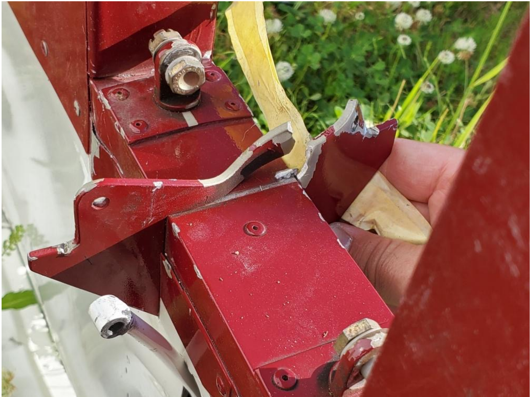
Photo 4 - Fractured stabilator control horn
