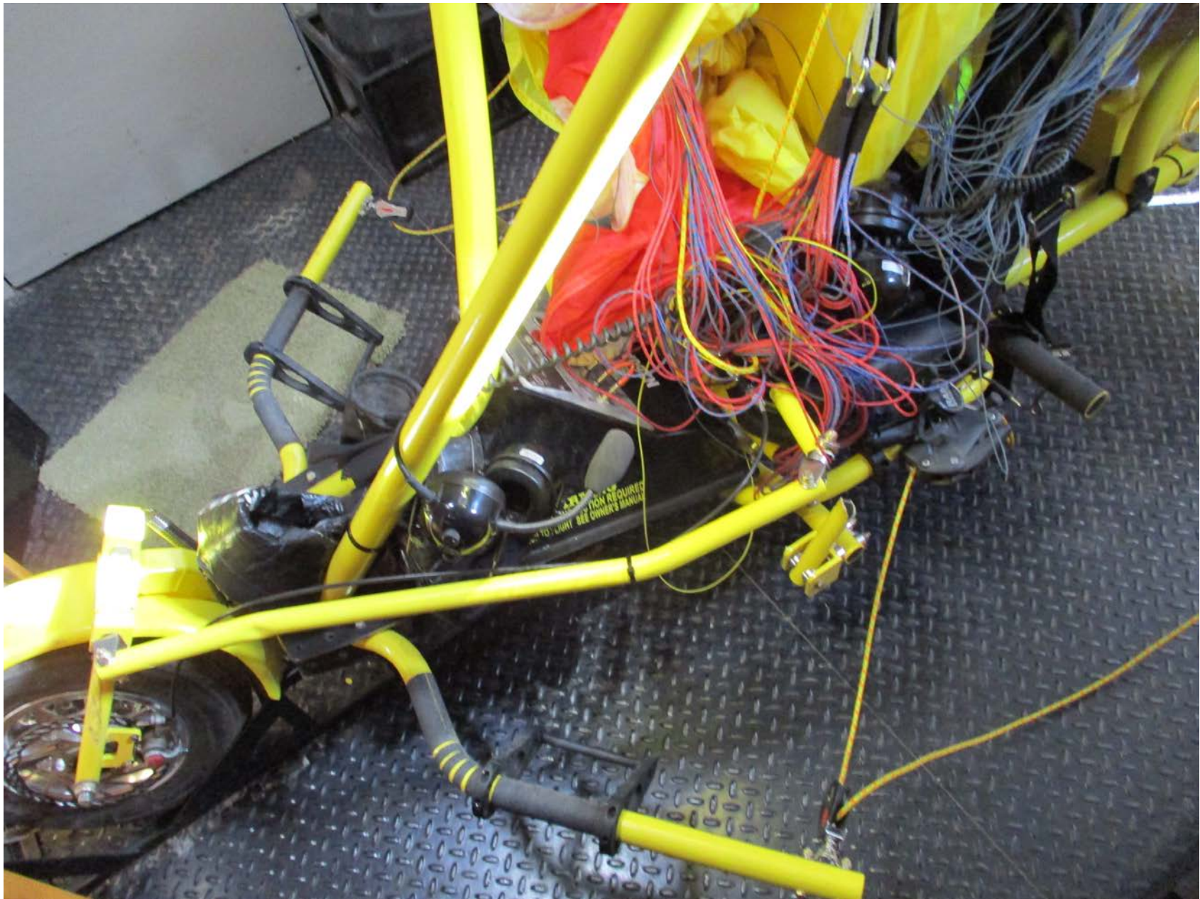
Photo 1 – Left Side View showing Steering Control damage
