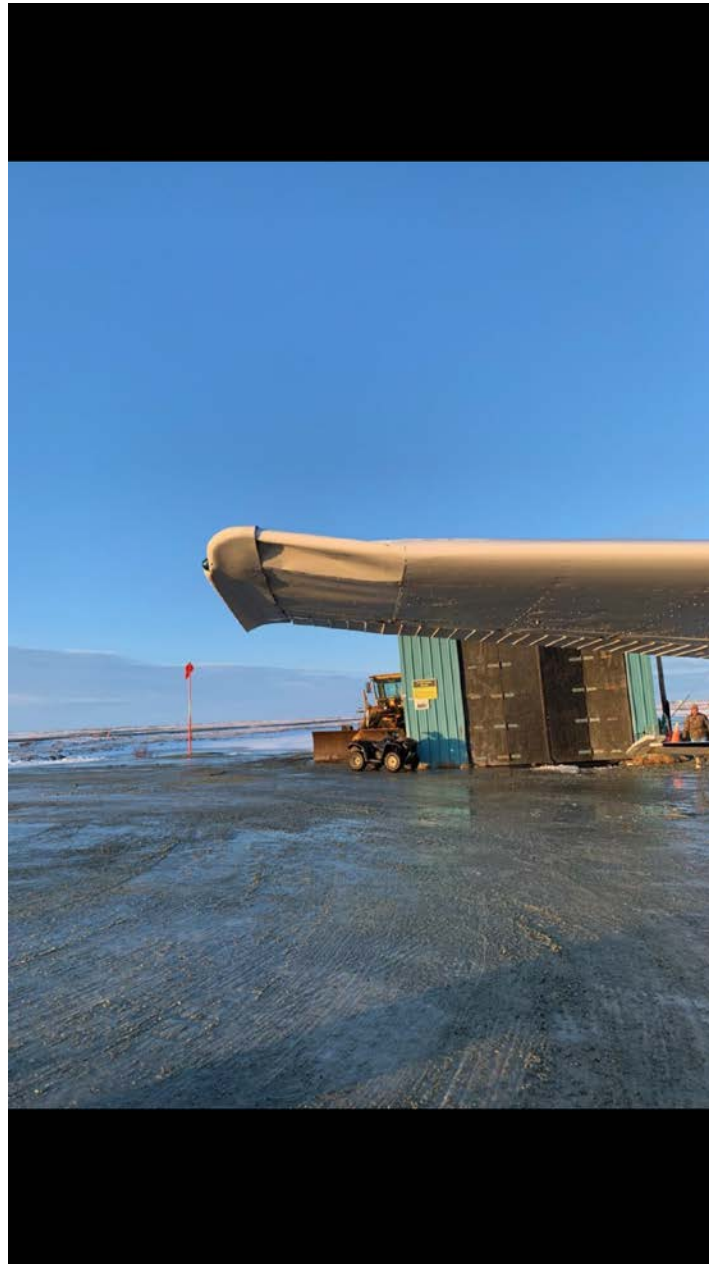
Photo 2 – Accident airplane’s damaged right wing.
