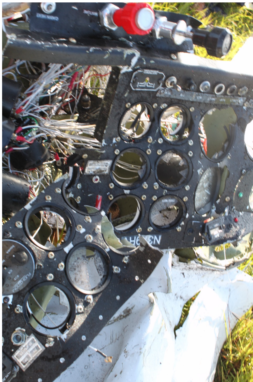
Photo 3 – View of damaged instrument panel
