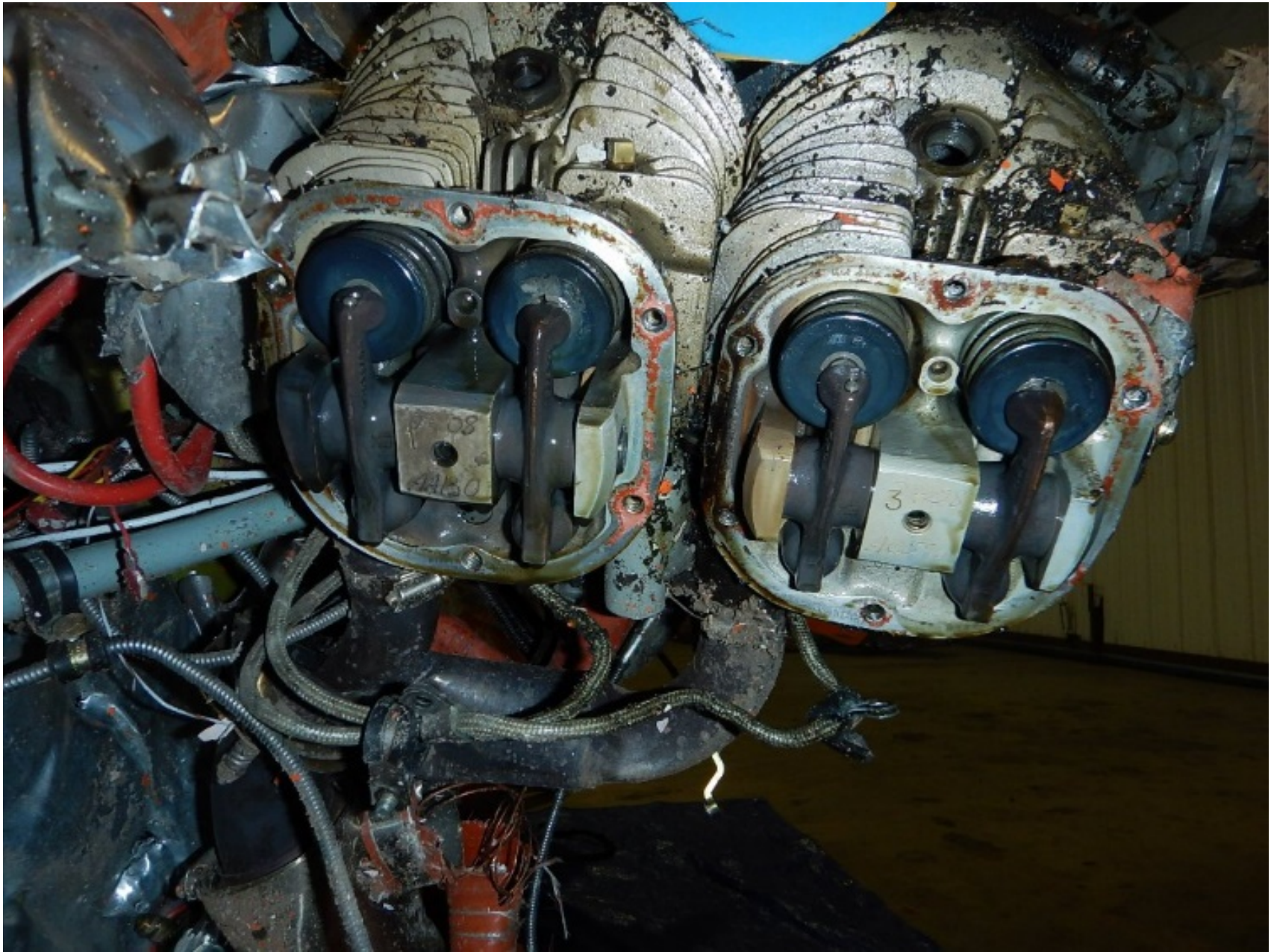
Photo 13 – Cylinders 1 and 3
