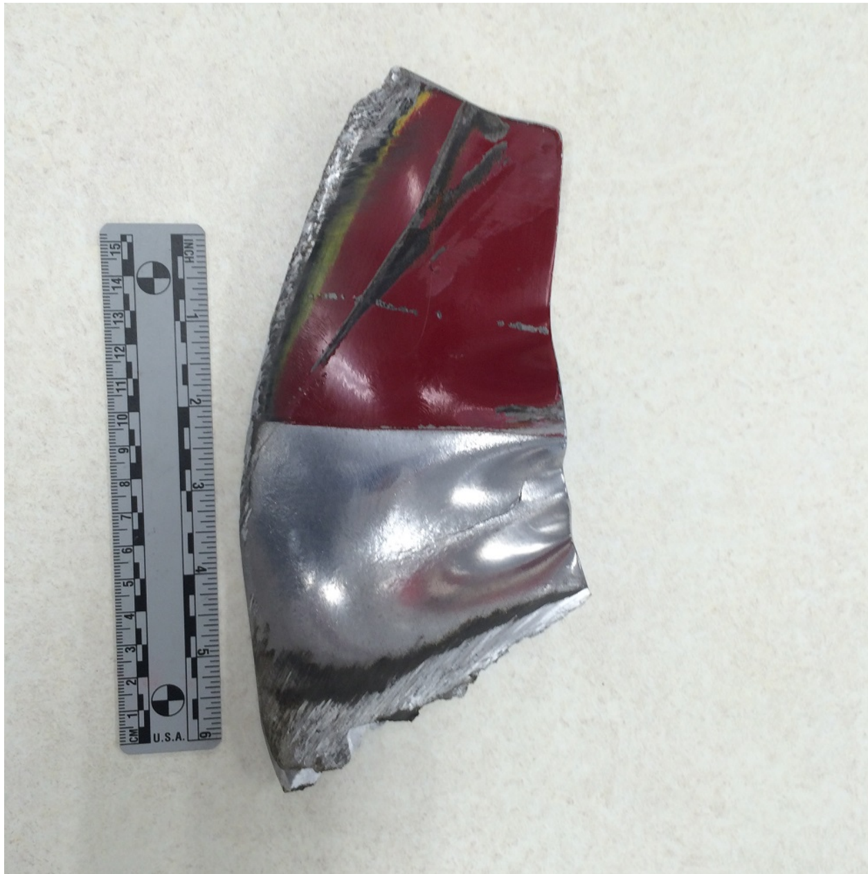
Photo 6 - Propeller tip
