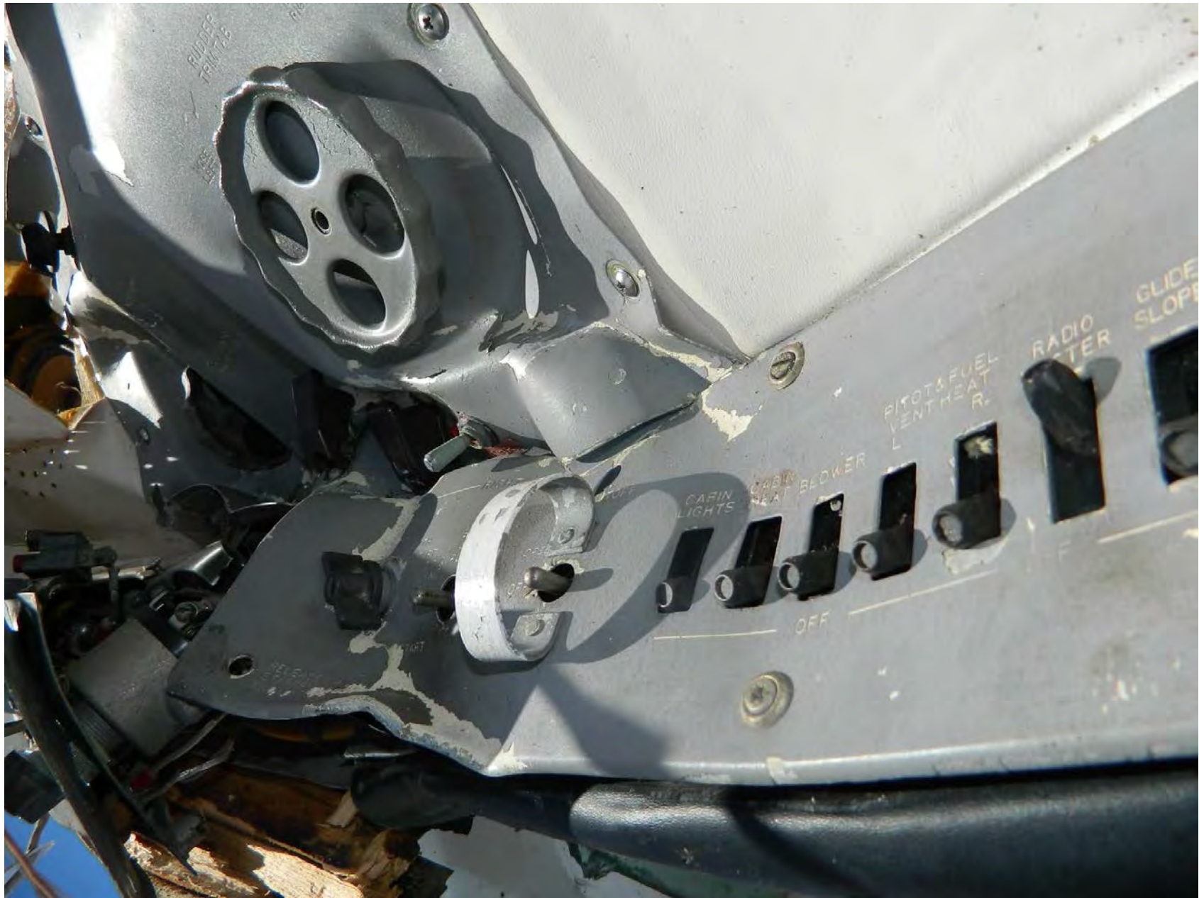
Photo 14 – Right Engine's Fuel and Ignition Switches
