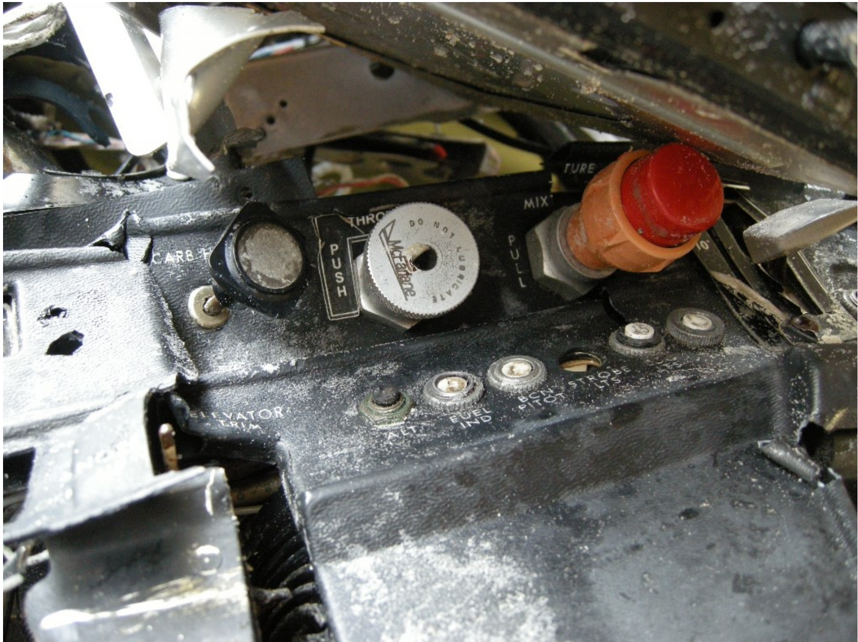
Photo 13 – Engine Controls (NTSB Photo)
