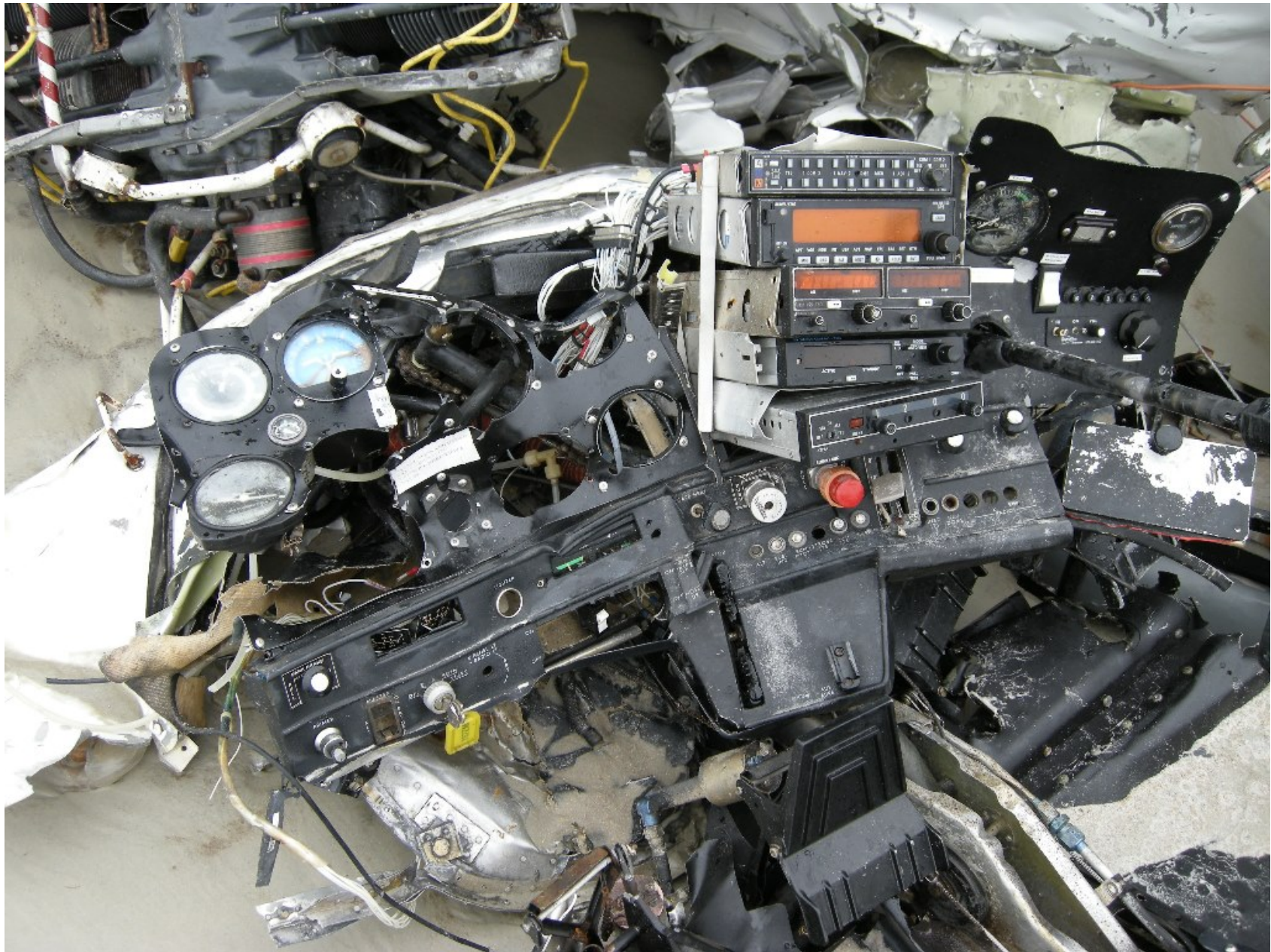
Photo 8 – Cockpit Area (NTSB Photo)
