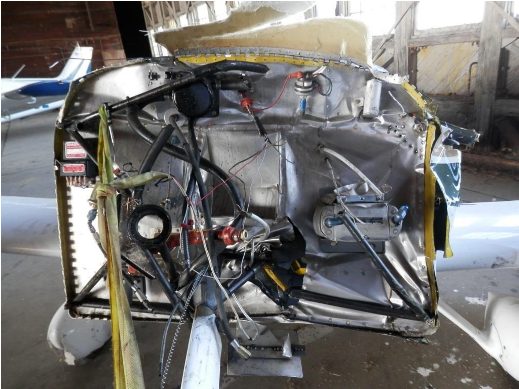
Photo 1 – Firewall and engine mount damage (Courtesy of FAA)
