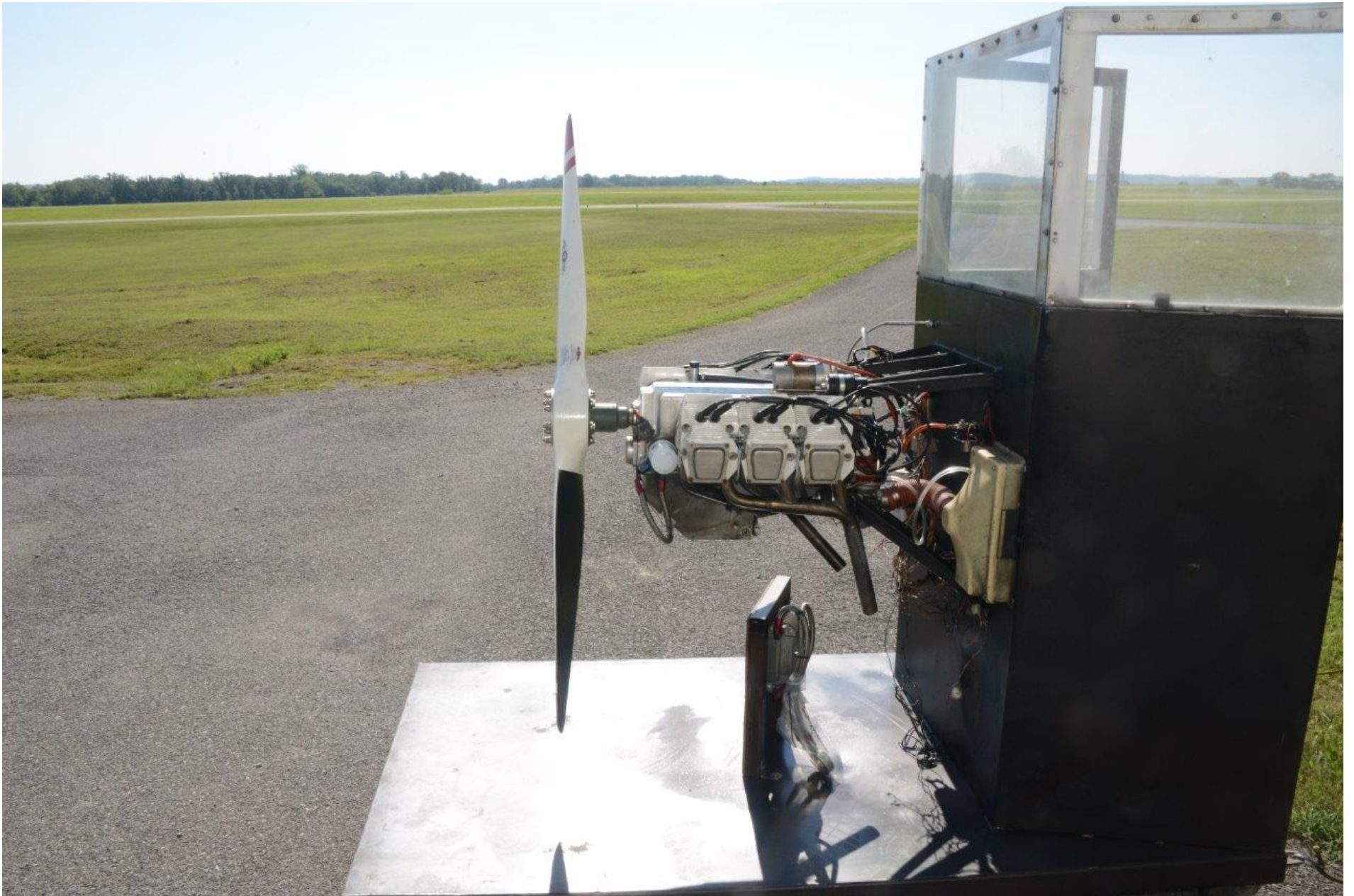
Photo 10 - View of the accident engine mounted on a test stand.
