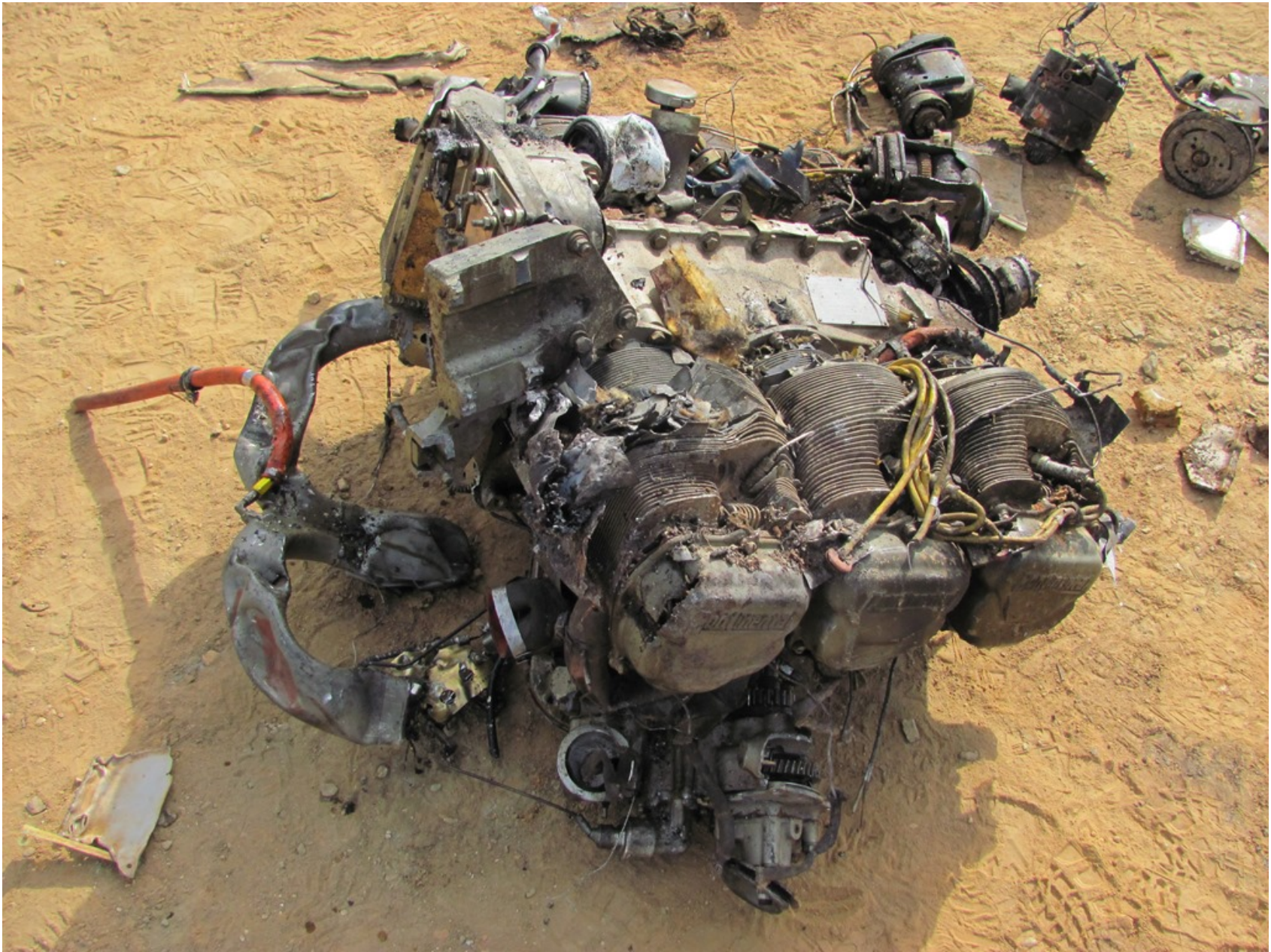
Photo 9 – Right side view of engine
