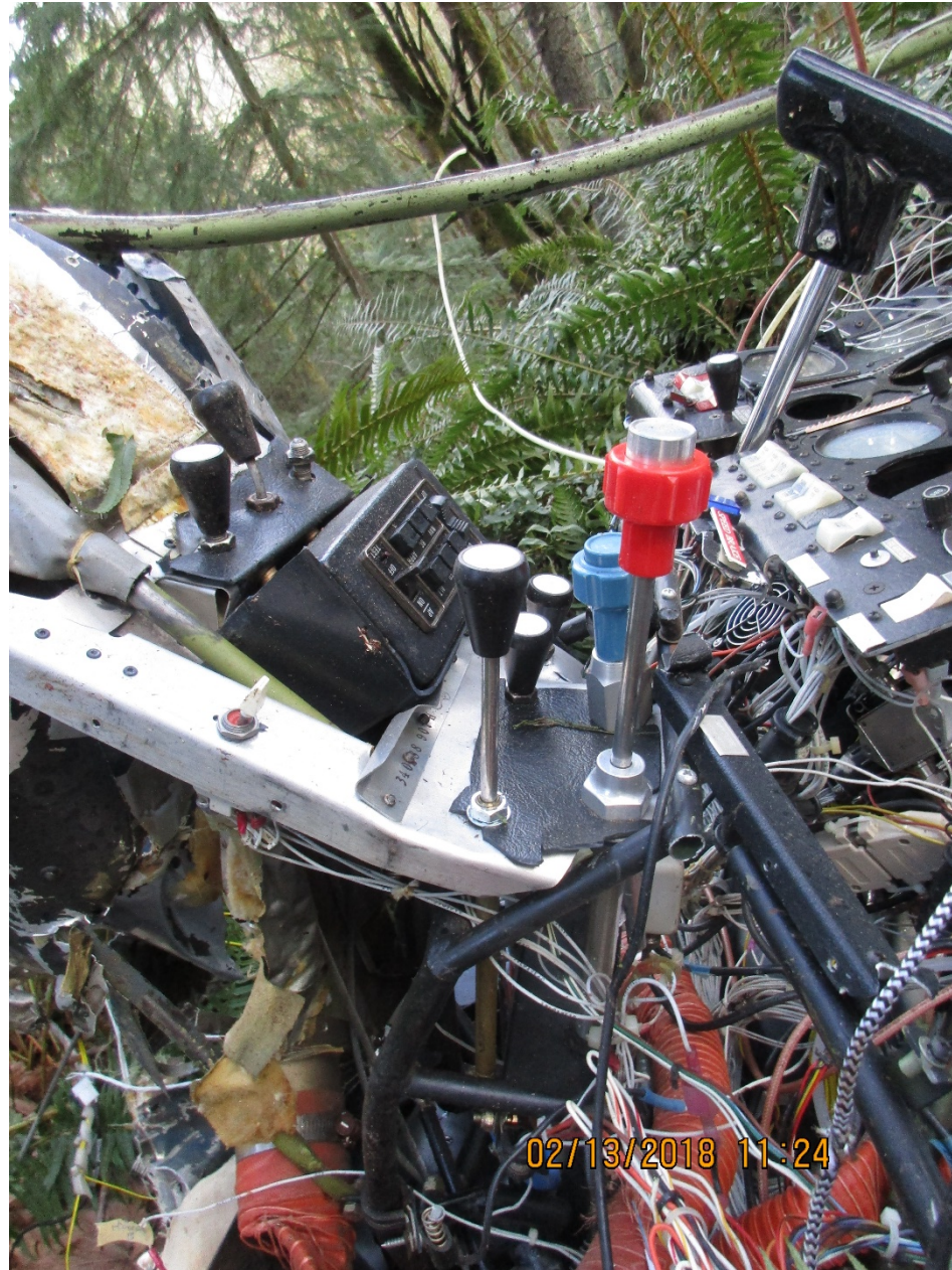
Photo 6 - Cockpit section indicating engine controls and instrument panel. (Courtesy of FAA)
