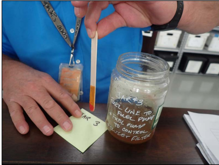
Figure 3: Color Change of Water Detecting Paste After Being Inserted in a Fuel Sample Collected from the Airplane
