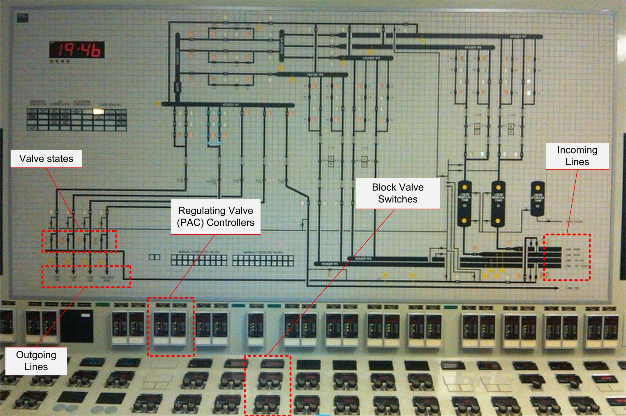
PHOTOGRAPH OF THE "MIMIC PANEL" AT MILPITAS TERMINAL Photograph of the Manual (MIMIC) Control panel from the Milpitas Terminal
